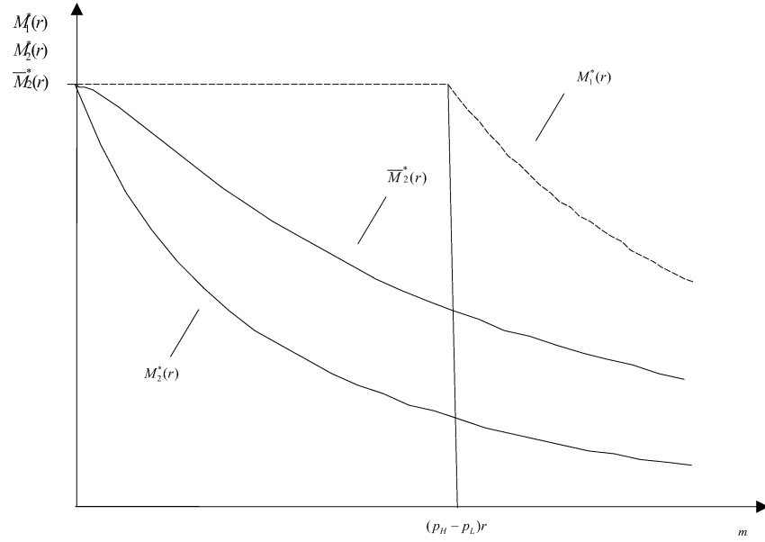
Fig. 2. Monitoring intensities in the single-bank and the two-bank game. The figure shows how the monitoring intensity M_1^*(r) of the single bank, the overall monitoring intensity \bar{M}_2^*(r) and the individual monitoring intensity M_2^*(r) of the two banks change as the cost of monitoring m increases. The loan rate is assumed to be the same in the two games, i.e., r_1 = r_2 = r .
