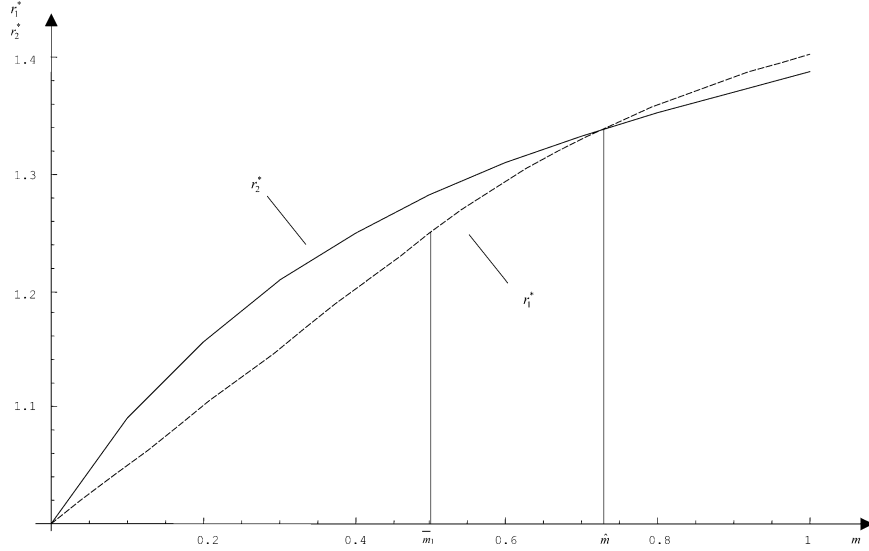
Fig. 5. Loan rates in the single-bank and the two-bank game for a high success probability of the project. The figure shows how the loan rates r_1^* of the single bank and r_2^* of the two banks change as the cost of monitoring m increases. The figure is drawn for a success probability p_L = 0.6 .
