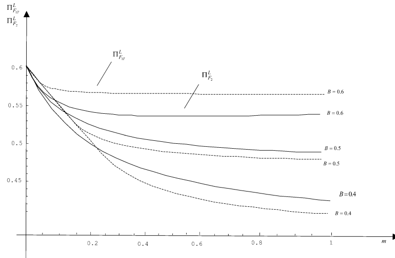
Fig. 10. Firm's expected profits with bank-investor and two-bank lending for a high success probability of the project. The figure shows how the firm's expected profits \Pi_{F_1}^L when it borrows from a single bank and outside investors and \Pi_{F_2}^L when it borrows from two banks change as the cost of monitoring m and the private benefit B increase. The figure is drawn for a success probability p_L = 0.6 .
