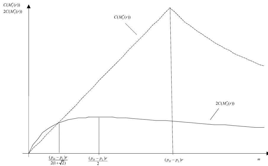
Fig. 3. Monitoring costs in the single-bank and the two-bank game. The figure shows how the monitoring costs C(M_1^*(r)) of the single bank and the total monitoring costs 2C(M_2^*(r)) of the two banks change as the cost of monitoring m increases. The loan rate is assumed to be the same in the two games, i.e., r_1 = r_2 = r .
