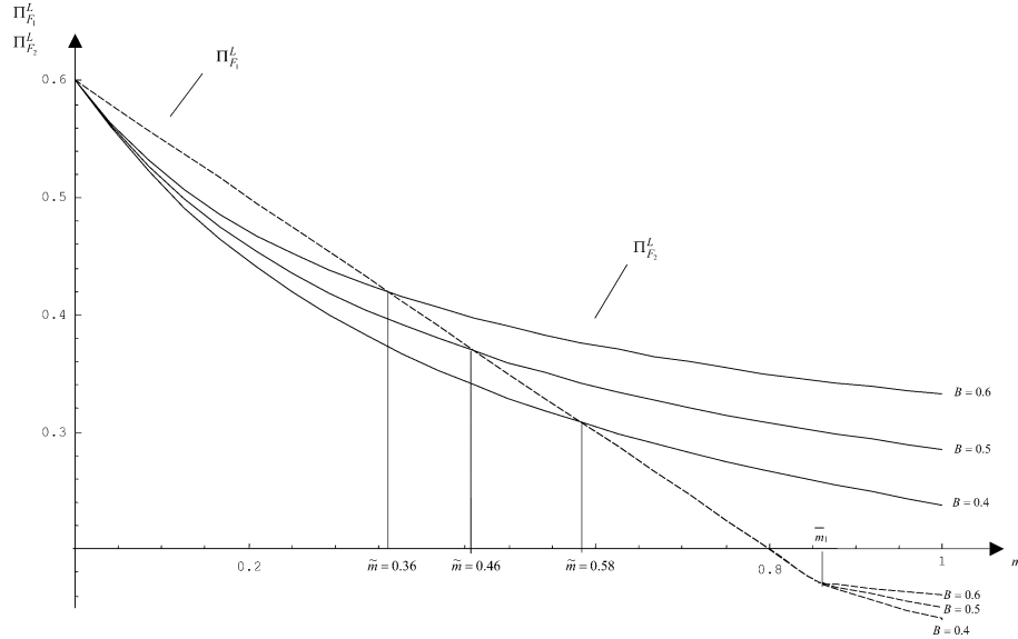
Fig. 6. Firm's expected profits with single-bank and two-bank lending. The figure shows how the firm's expected profits \Pi_{F_1}^L when it borrows from a single bank and \Pi_{F_2}^L when it borrows from two banks change as the cost of monitoring m and the private benefit B increase. The figure is drawn for a success probability of the project p_L = 0.4 .
