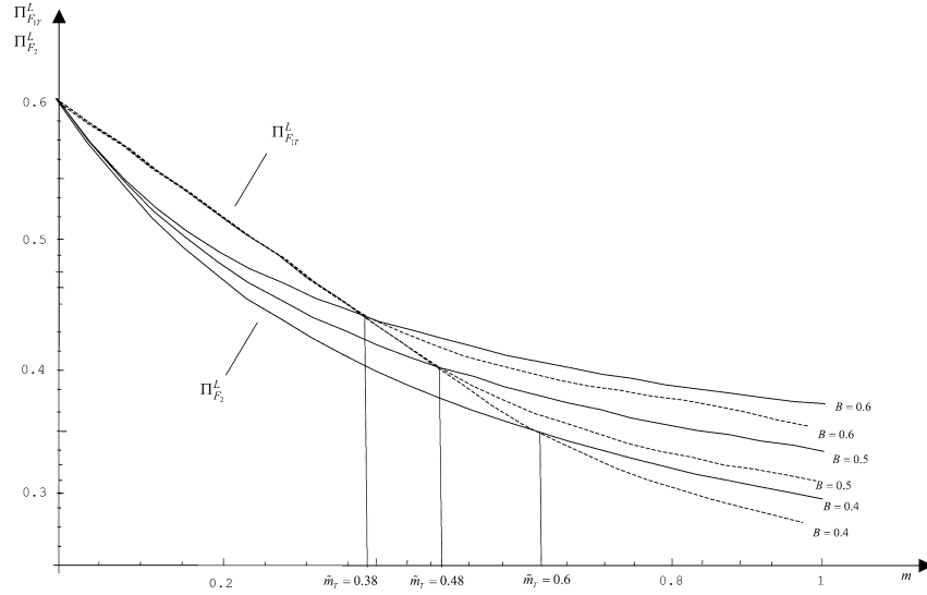
Fig. 9. Firm's expected profits with bank-investor and two-bank lending for a low success probability of the project. The figure shows how the firm's expected profits \Pi_{F_1}^L when it borrows from a single bank and outside investors and \Pi_{F_2}^L when it borrows from two banks change as the cost of monitoring m and the private benefit B increase. The figure is drawn for a success probability p_L = 0.4 .
